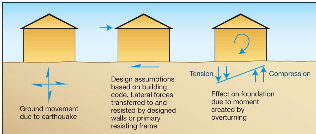
Figure 4-21. Seismic design causes and effects
