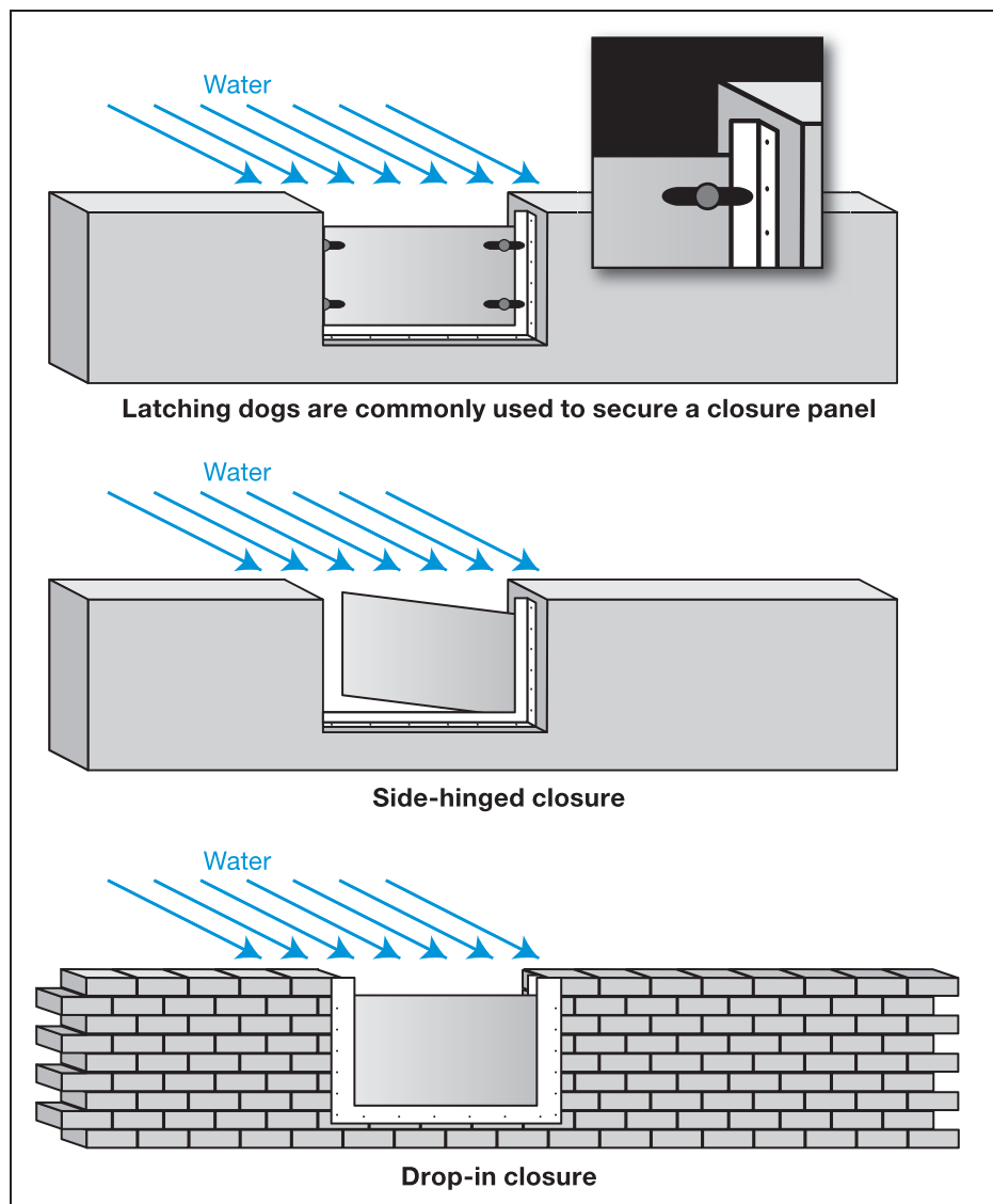
Figure 5F-17. Typical floodwall closures
