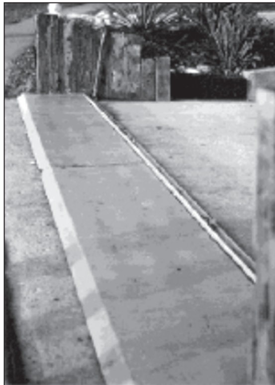
Figure 5D-4. A shield hinged at its bottom could prevent low-level flooding from entering a garage or driveway.
