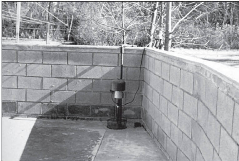
Figure 6-54. Interior sump pump for a residential floodwall
